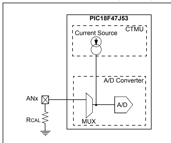
FIGURE 27-2: CTMU CURRENT SOURCE CALIBRATION CIRCUIT
