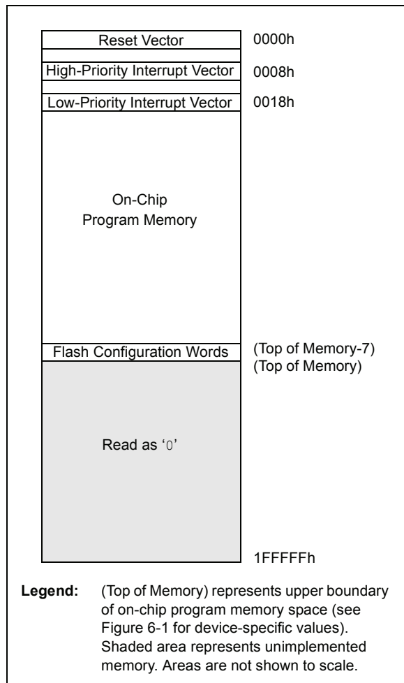
FIGURE 6-2: HARD VECTOR AND CONFIGURATION WORD LOCATIONS FOR PIC18F47J53 FAMILY DEVICES
