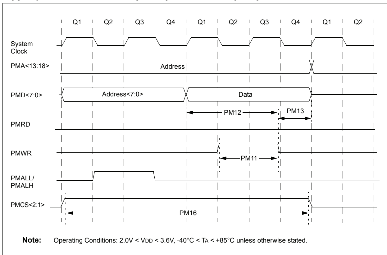
FIGURE 31-11: PARALLEL MASTER PORT WRITE TIMING DIAGRAM
