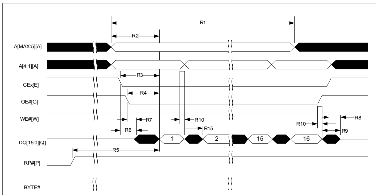
Figure 14: 16-Word Asynchronous Page Mode Read
