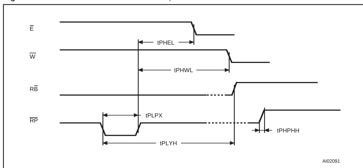
Figure 9. Read and Write AC Characteristics, \overline{R} Related
