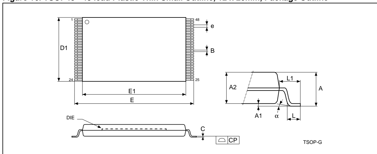
Figure 16. TSOP48 - 48 lead Plastic Thin Small Outline, 12 x 20mm, Package Outline
