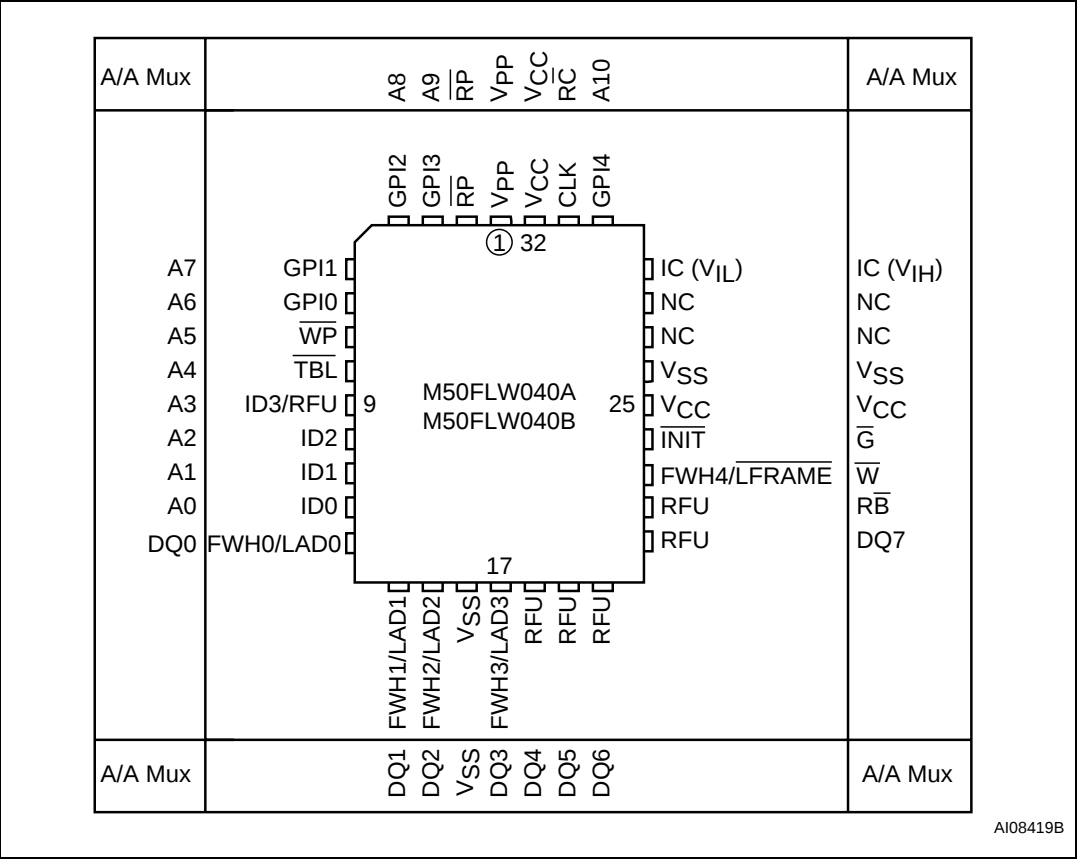
Figure 3. PLCC connections
