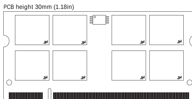
Figure 1: 200-Pin SODIMM (MO-224 R/C E)
