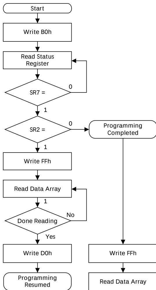
Figure 13: PROGRAM SUSPEND/RESUME
