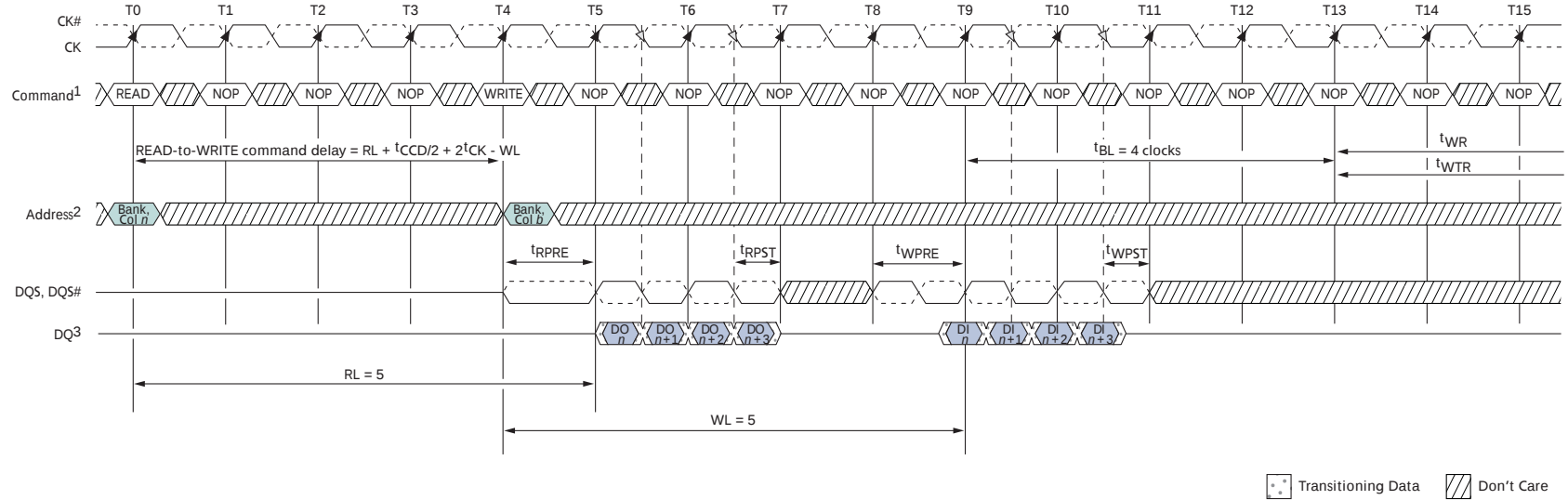
Figure 71: READ (BC4) to WRITE (BC4) OTF
