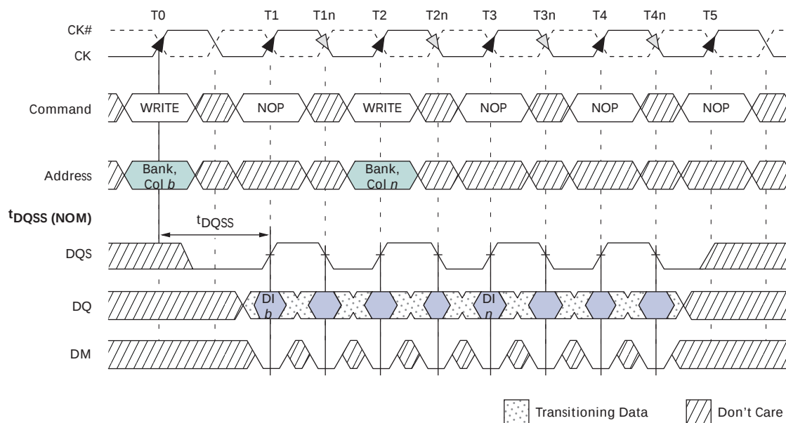
Figure 39: Consecutive WRITE-to-WRITE
