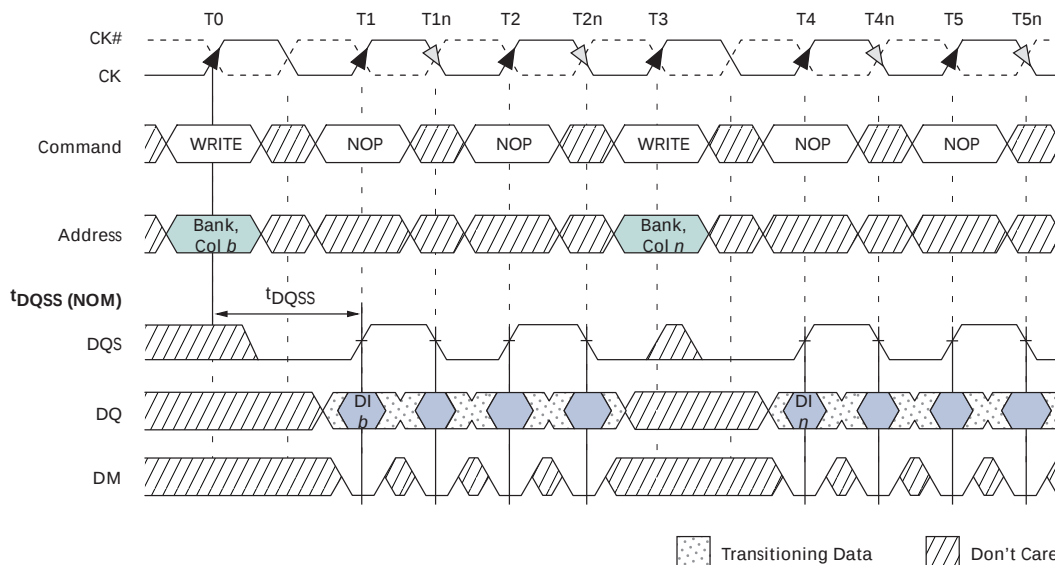
Figure 40: Nonconsecutive WRITE-to-WRITE
