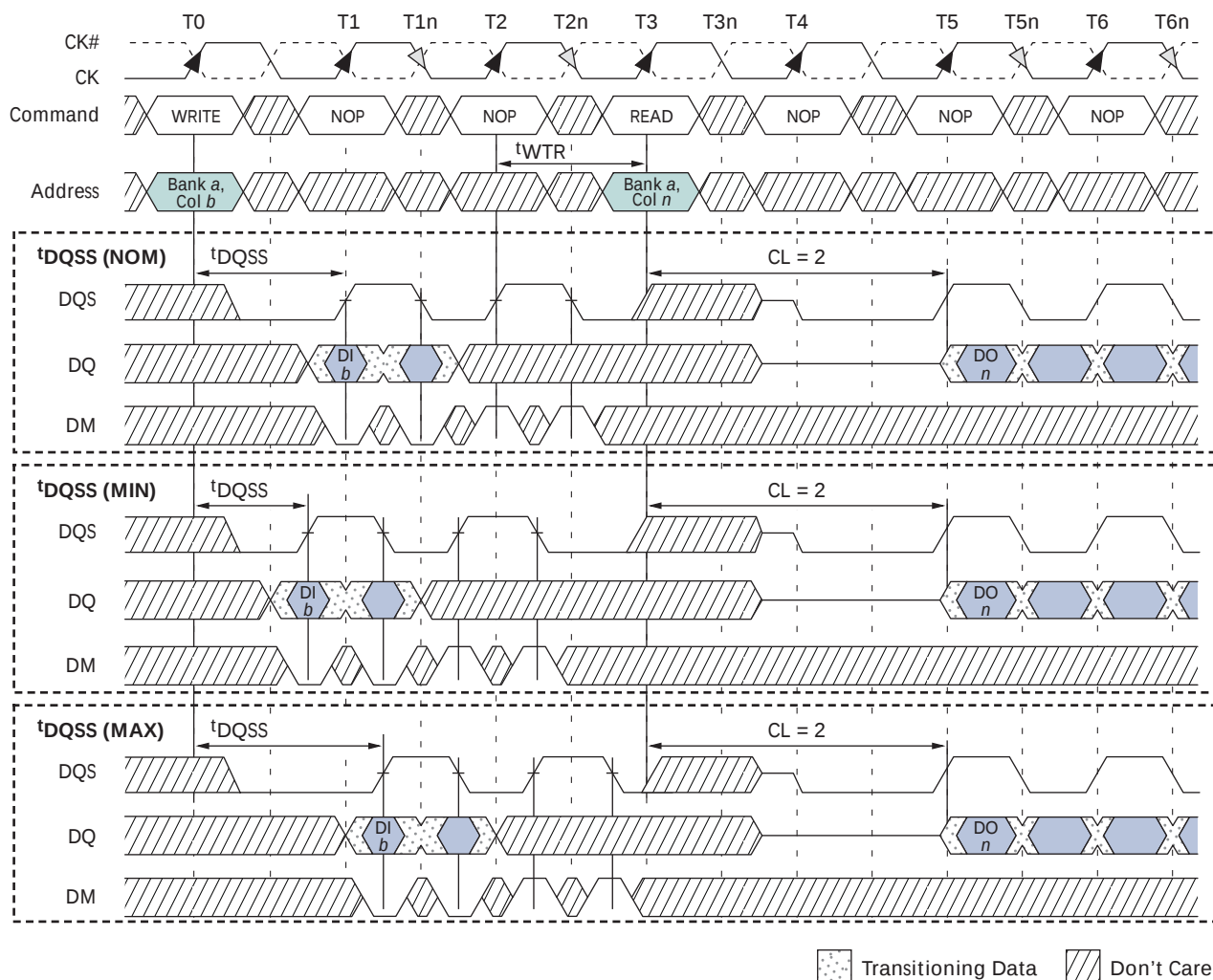
Figure 43: WRITE-to-READ – Interrupting
