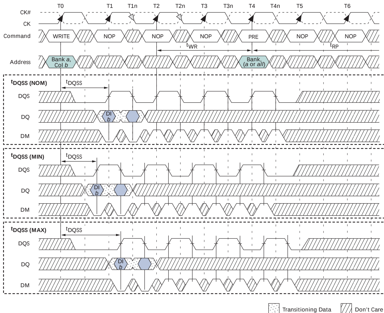
Figure 46: WRITE-to-PRECHARGE – Interrupting
