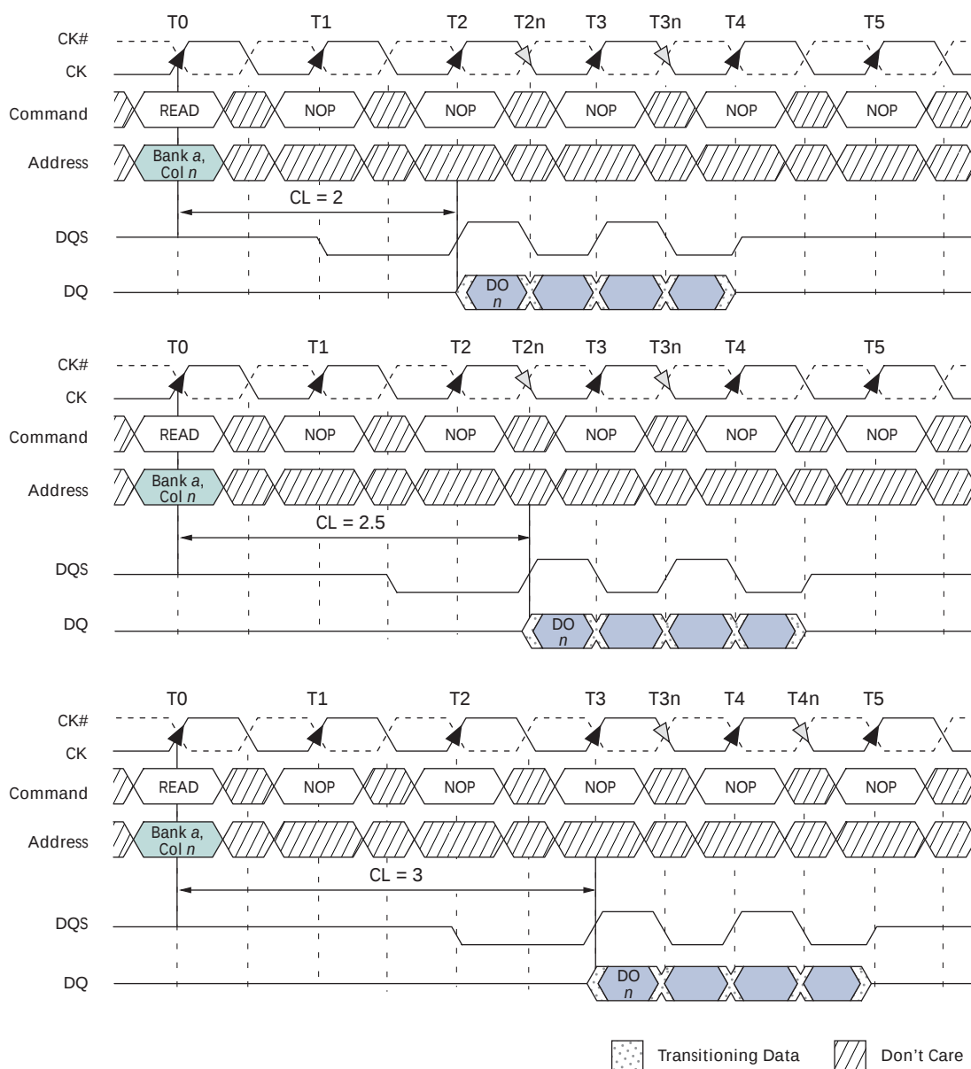
Figure 27: READ Burst
