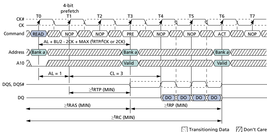
Figure 50: READ-to-PRECHARGE – BL = 4
