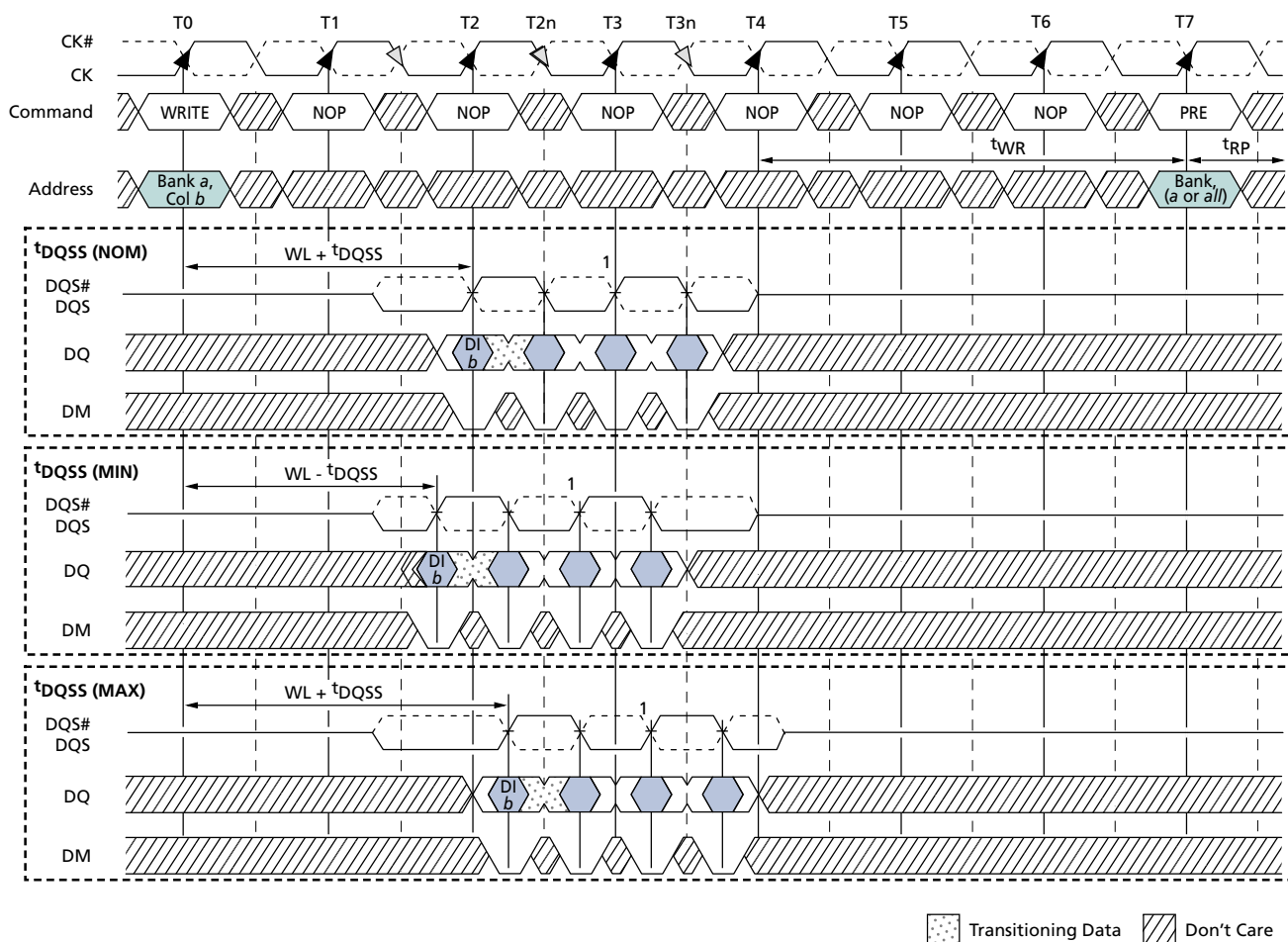
Figure 61: WRITE-to-PRECHARGE
