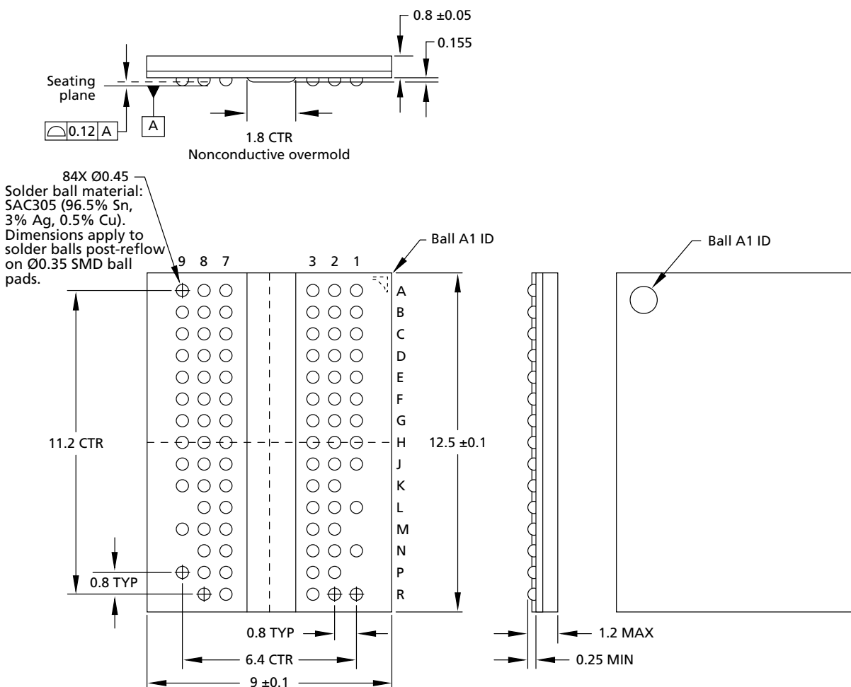
Figure 8: 84-Ball FBGA Package (9mm x 12.5mm) – x16
