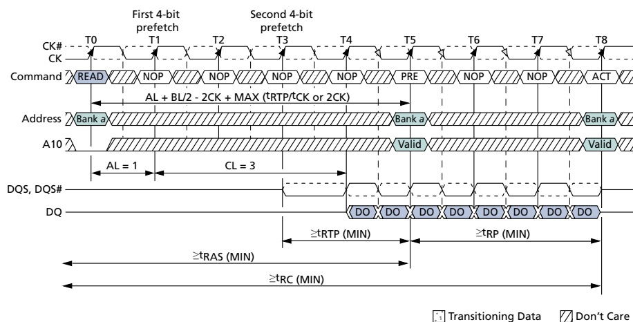
Figure 50: READ-to-PRECHARGE – BL = 8
