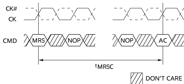
Figure 8: Mode Register Set Timing
