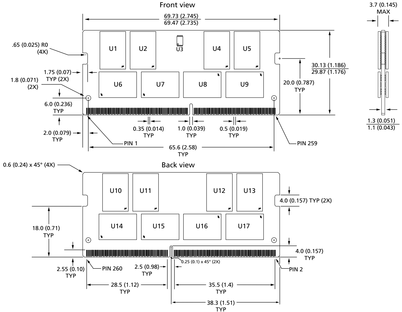
Figure 5: 260-Pin DDR4 SODIMM, R/C-B1 (PCB 1855)
