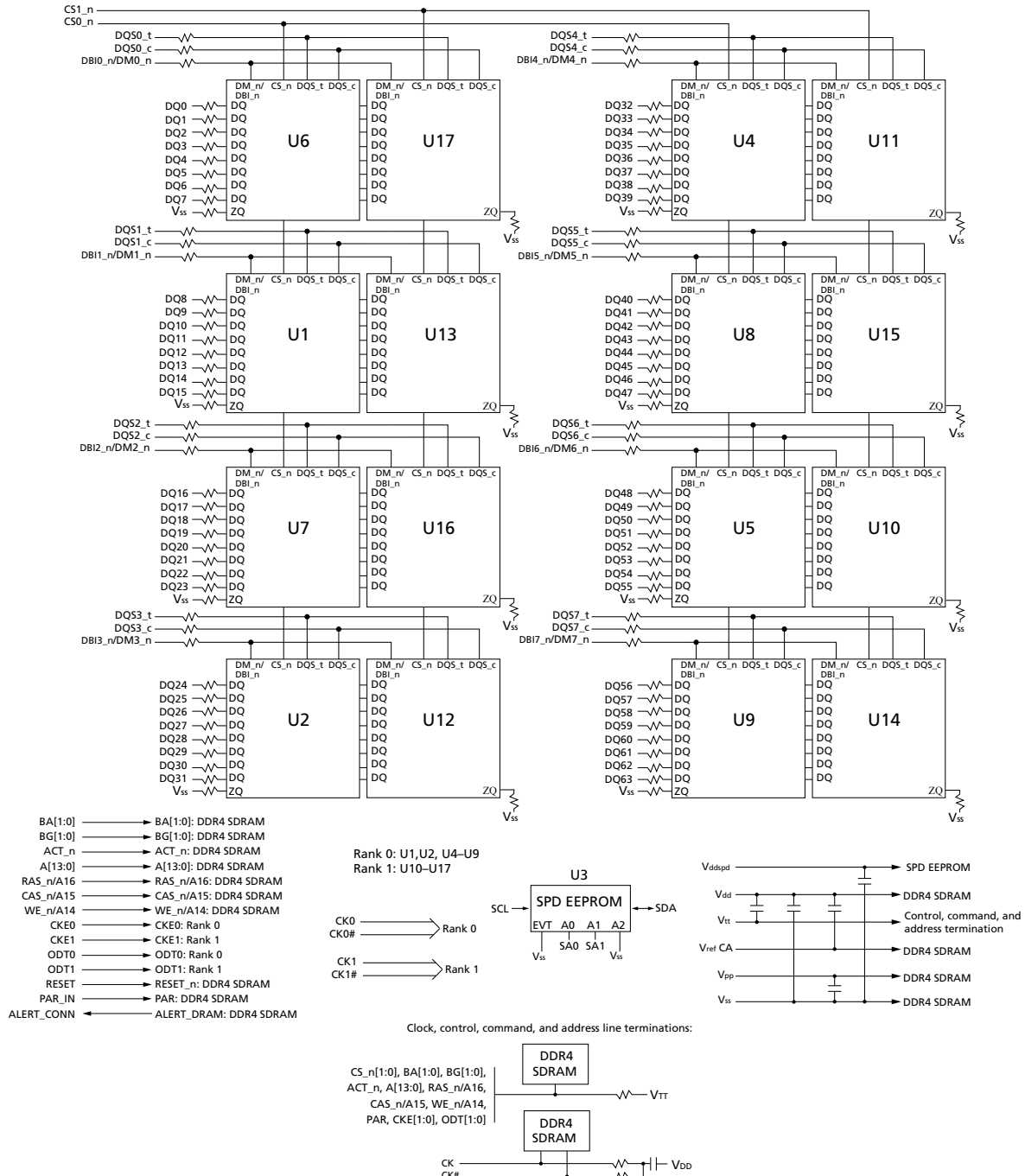
Figure 3: Functional Block Diagram, R/C-B1 (PCB 1850)
