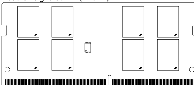
Figure 2: 260-Pin SODIMM (MO-310, R/C E1)
