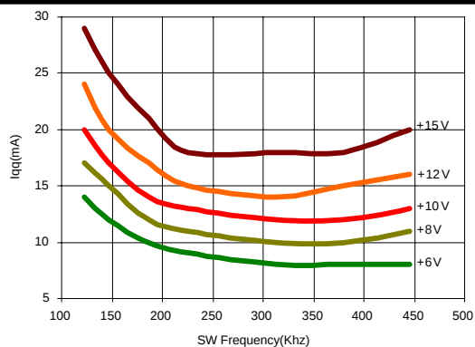
IQQ (POS) VS. SW FREQUENCY
