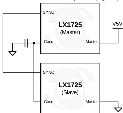
Figure 2 – Two Devices Synchronized Block Diagram
