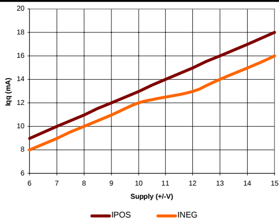
IQQ VS. SUPPLY VOLTAGE
