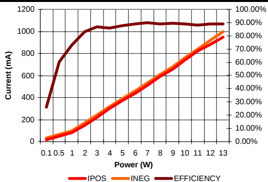
EFFICIENCY @ 80HM LOAD
