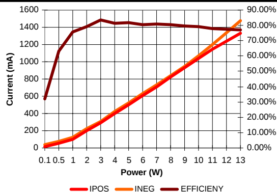
EFFICIENCY @ 40HM LOAD
