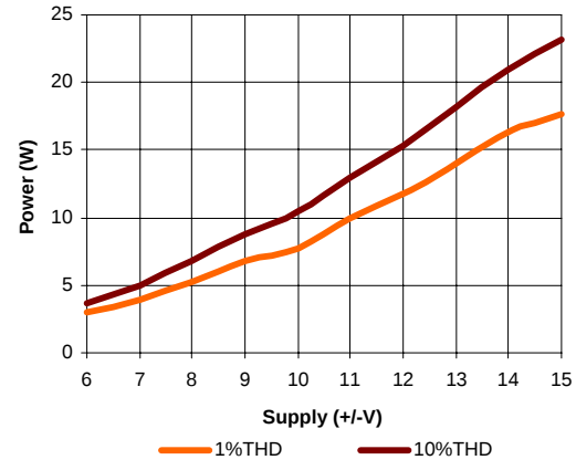
POWER VS. SUPPLY @40HM
