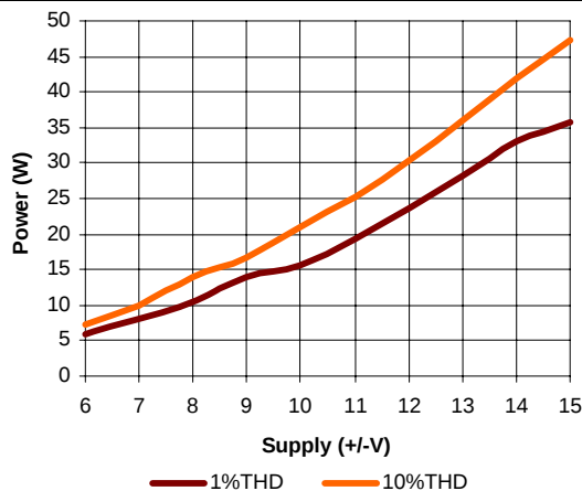
POWER VS. SUPPLY @80HM BTL
