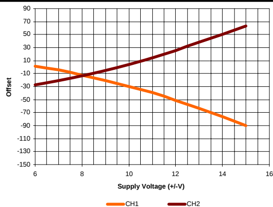
DC OFFSET @ SUPPLY
