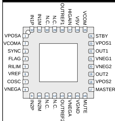
LQ PACKAGE (Top View)
