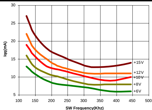
IQQ (NEG) VS. SW FREQUENCY
