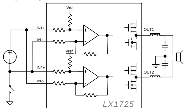
Figure 6 – Audio Input Block Diagram
