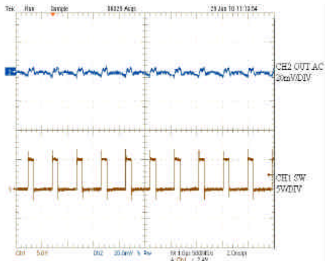
Figure 7 - Output ripple
