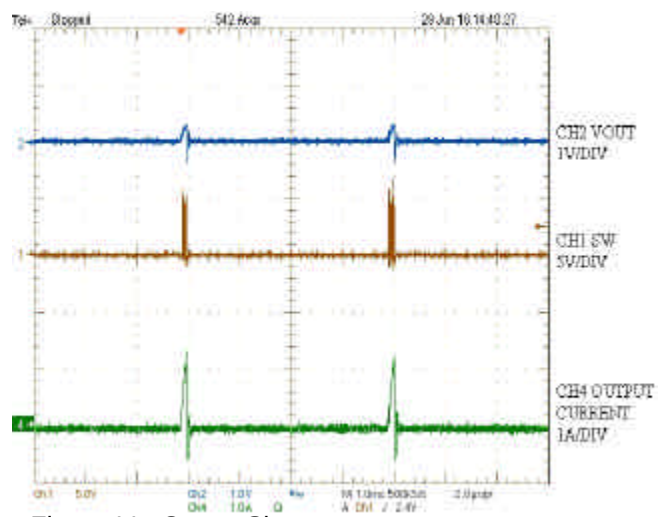
Figure 11 - Output Short
