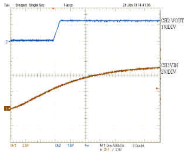
Figure 9 - Startup
