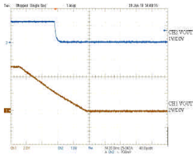
Figure 10 - Shutdown
