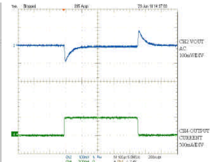
Figure 8 - Transient response
