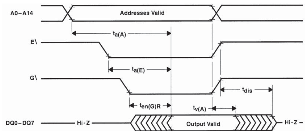
FIGURE 3. READ-CYCLE TIMING
