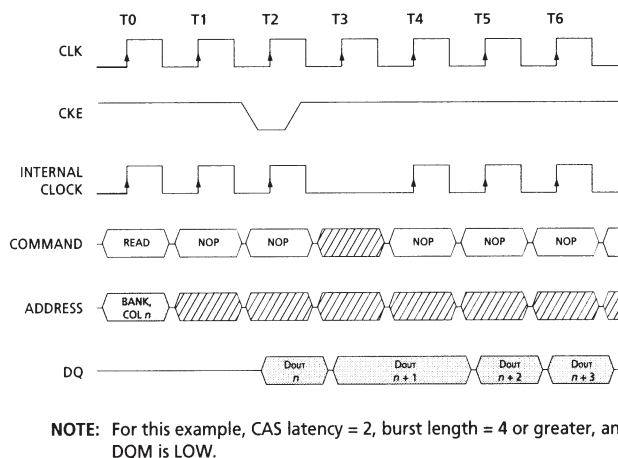
FIGURE 23: Clock Suspend During READ Burst
