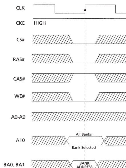
FIGURE 20: PRECHARGE Command
