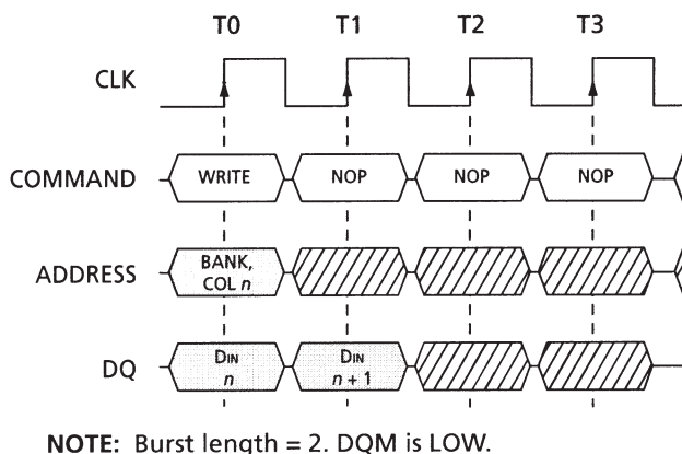
FIGURE 14: WRITE Burst
