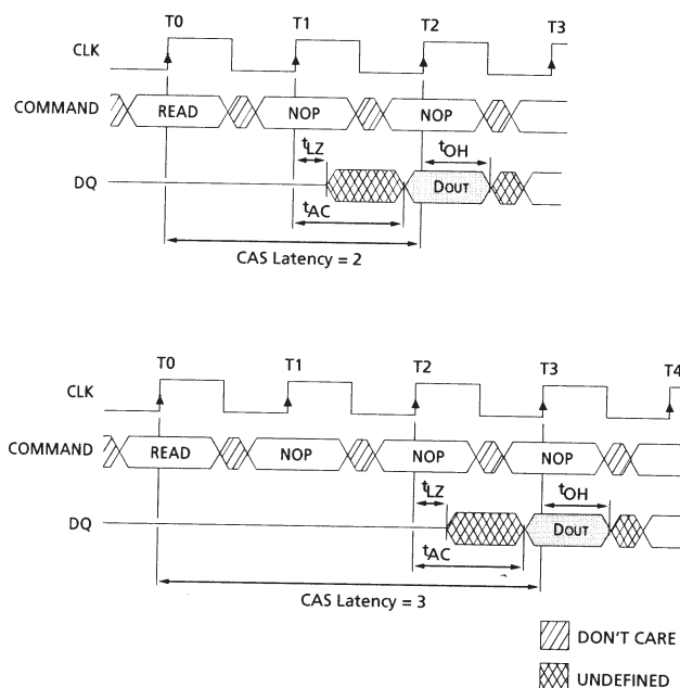
FIGURE 6: CAS Latency
