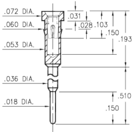
1261-0-15-XX-30-XX-04-0 Press-fit in .057 mounting hole
