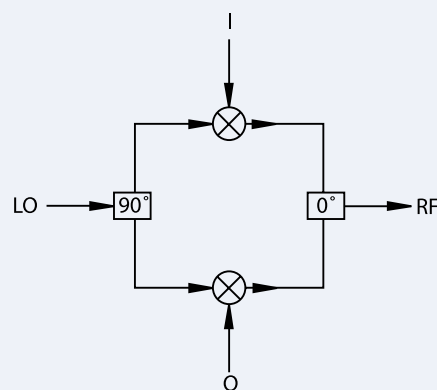
I&Q modulation block diagram
