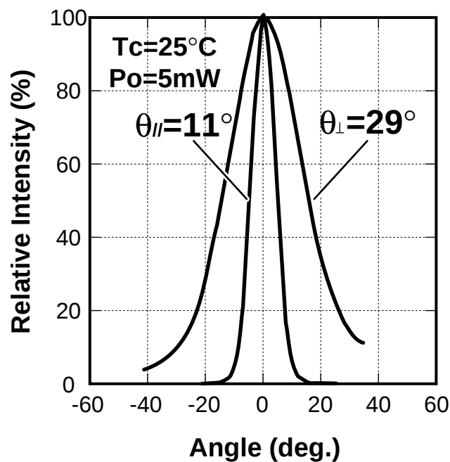
Far-Filed-Patterns
