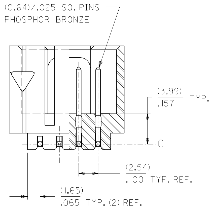
SECTION E-E
