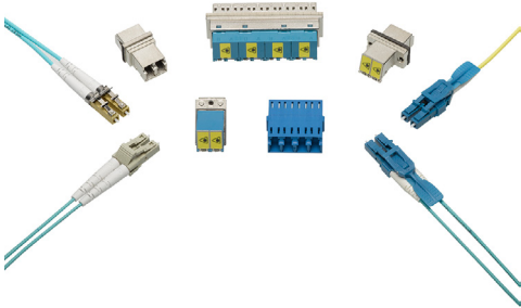
LC Connectors and Adapters
