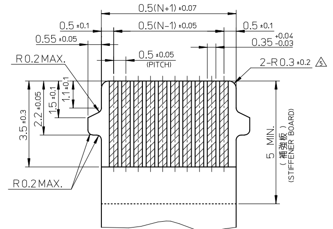
適合FPC推奨寸法 APPLICABLE FPC RECOMMENDED DIMENSION
