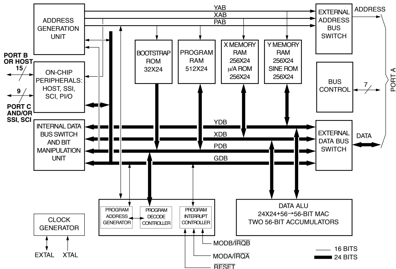
Figure 1. DSP56001 Block Diagram
