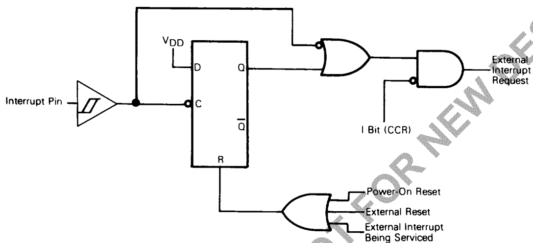
FIGURE 16 — EXTERNAL INTERRUPT
