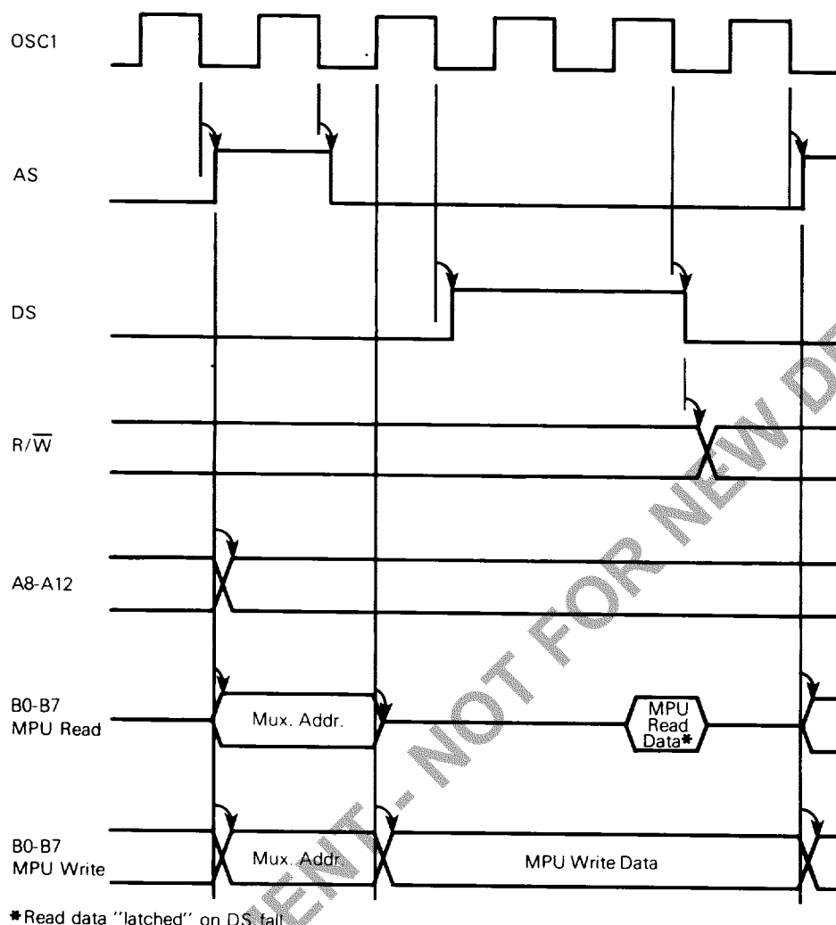
FIGURE 9 — OSC1 TO BUS TRANSITIONS
