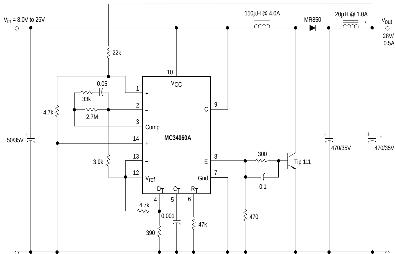
Figure 20. Step-Up Converter
