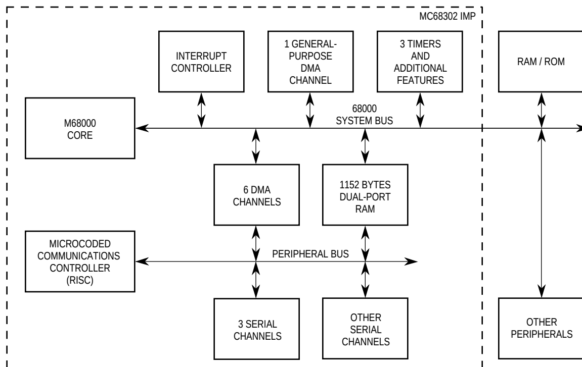
Figure 1-3. MC68302 System Design
