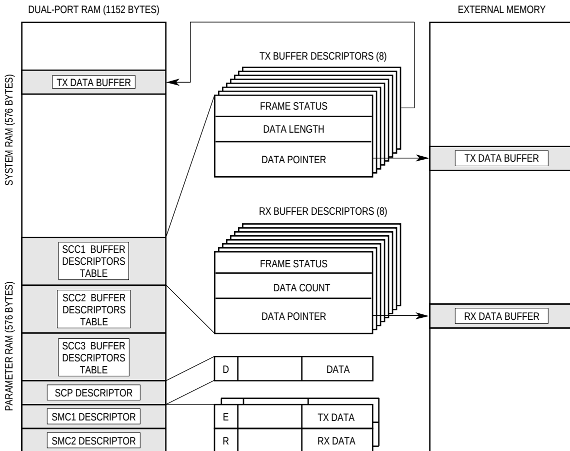
Figure 4-15. Memory Structure
