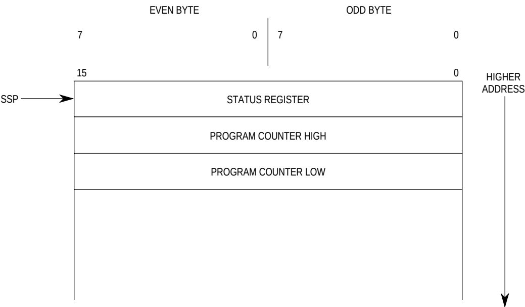
Figure 2-4. M68000 Short-Form Exception Stack Frame
