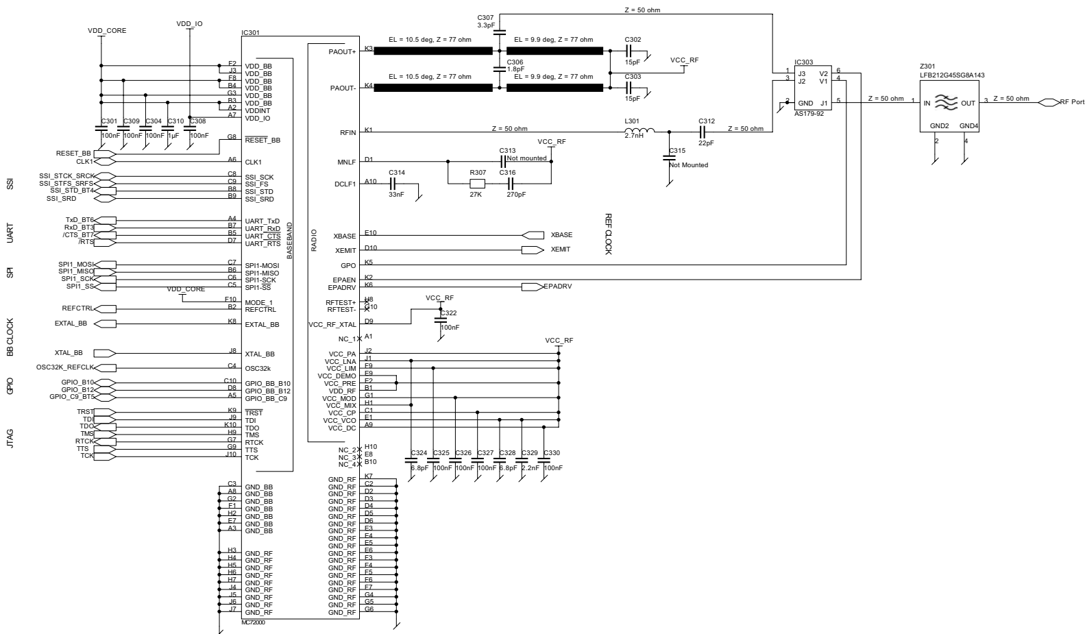
Figure 92. Application Example Evaluation Schematic
