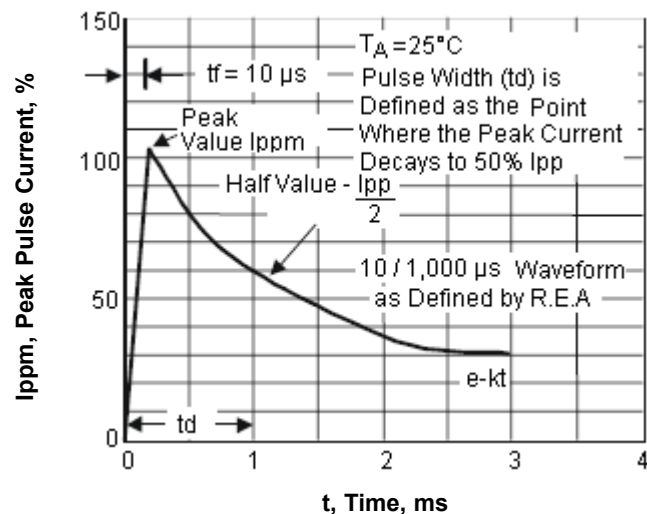
Fig. 3-Pulse Waveform
