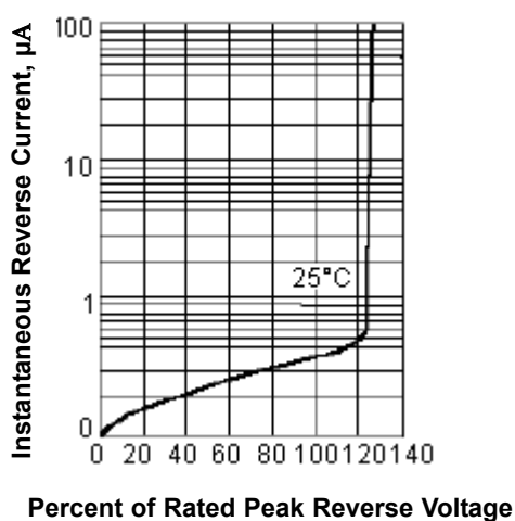
Figure 4 - Reverse Characteristics
