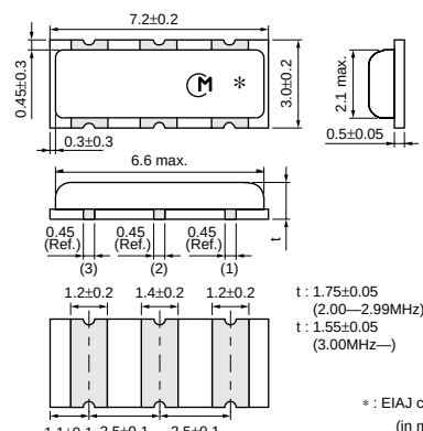
CSTCC_G(A) 2.00-3.99MHz
