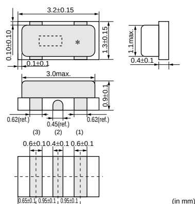
CSTCE_V 12.51-19.99MHz
