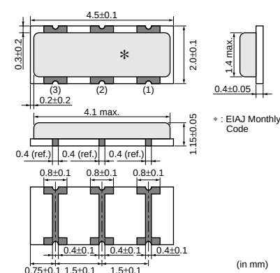
CSTCR_G(A) 4.00-7.99MHz
