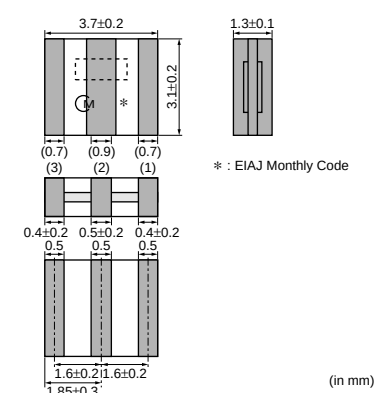
CSTCV_X_Q 14.70-70.00MHz
