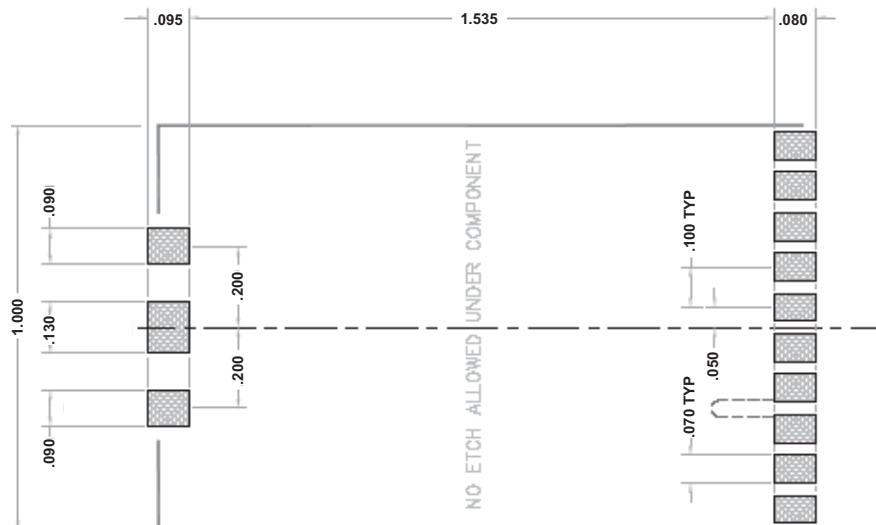
DM1800-916MN SMT Mounting Pattern
