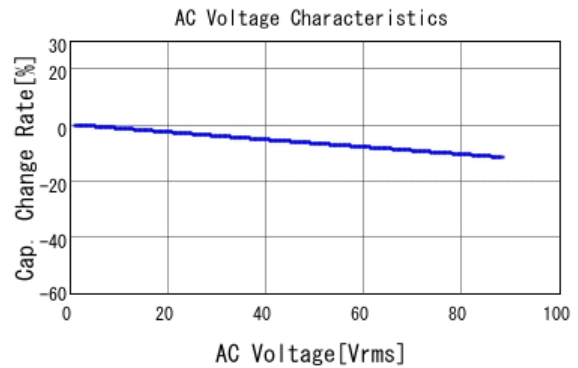
■ GRM32QR72E154KW01 C-AC Voltage capchange, DCOV, 25.0d
