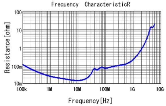
■ GRM32QR72E154KW01 R DCOV, 25degC
