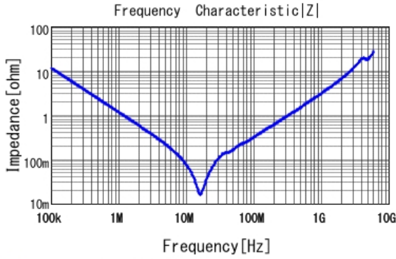
■ GRM32QR72E154KW01 |Z| DCOV, 25degC
