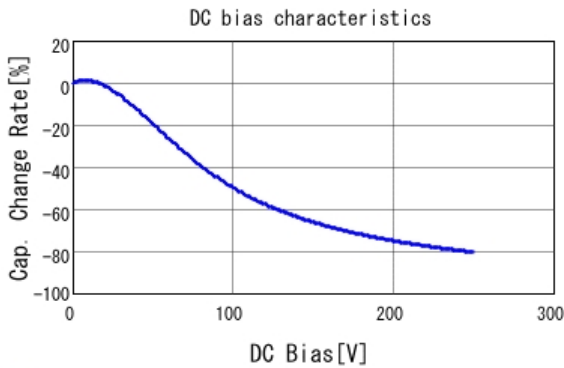
■ GRM32QR72E154KW01 C-DC bias capchange, 25.0degC, AC1V
