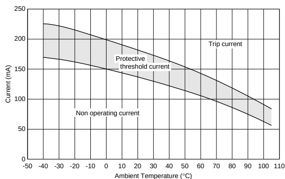
PTGL5SAS270K6B51B0
