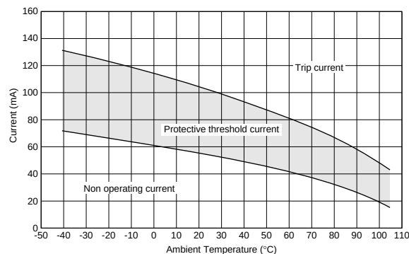
PRG21AR420MS1RA
