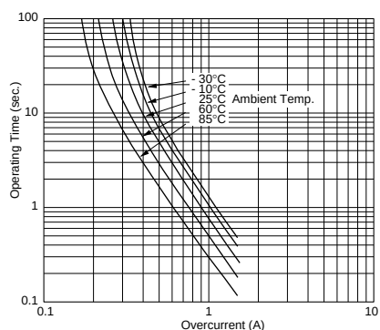
PTGL5SAS100K4B51B0
