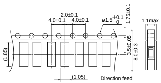
PR*18_RB Series: Paper Tape
