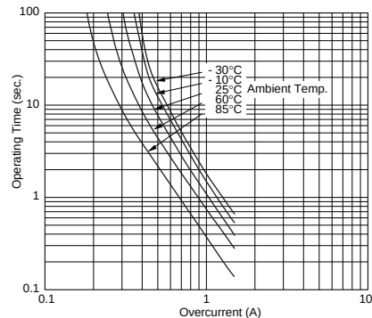
PTGL5SAS6R8K3B51B0
