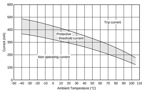
PTGL9SAS7R6K6B51B0
