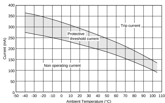
PTGL5SAS100K4B51B0
