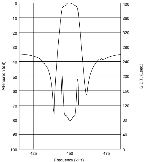
SFPKA450KG1A-R1
