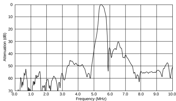
SFSRA5M50DF00-B0
