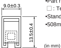
Magazine Dimensions
