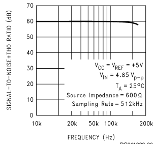
Signal-to-Noise + THD Ratio vs Signal Frequency
