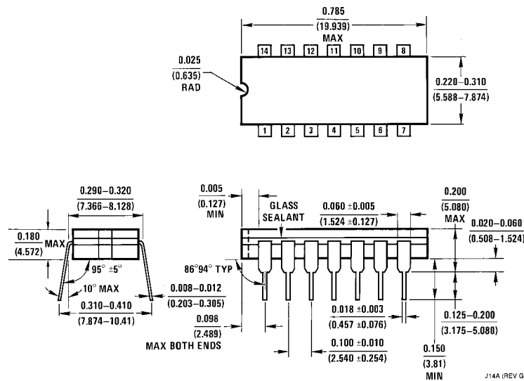
14-Lead Ceramic Dual-In-Line Package (J) Order Number 54LS164DMQB or DM54LS164J NS Package Number J14A
