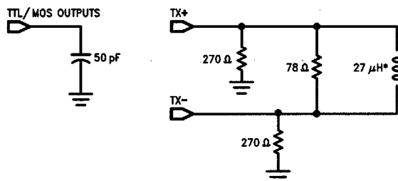
FIGURE 12. Test Loads
