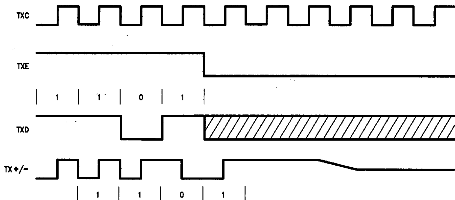
FIGURE 6. Transmit Timing - End of Transmission (last bit = 1)
