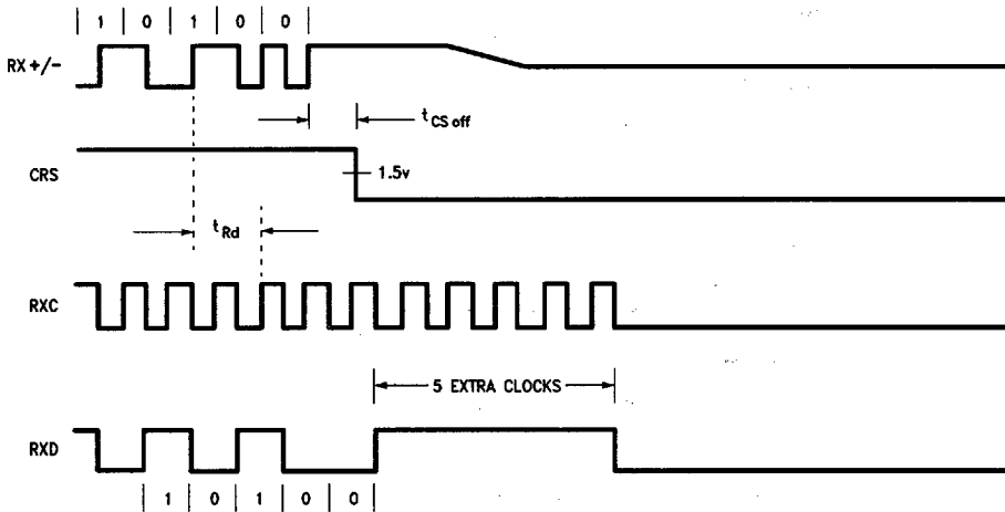
FIGURE 8. Receive Timing - End of Packet (last bit = 0)
