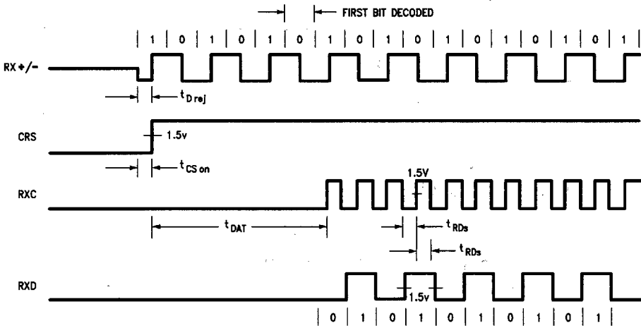
FIGURE 7. Receive Timing - Start of Packet
