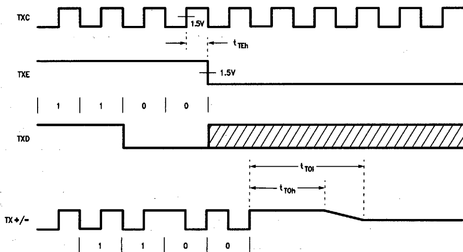
FIGURE 5. Transmit Timing - End of Transmission (last bit = 0)
