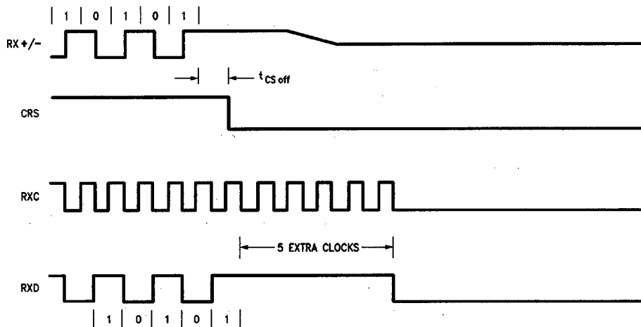
FIGURE 9. Receive Timing - End of Packet (last bit = 1)
