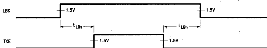
FIGURE 11. Loopback Timing
