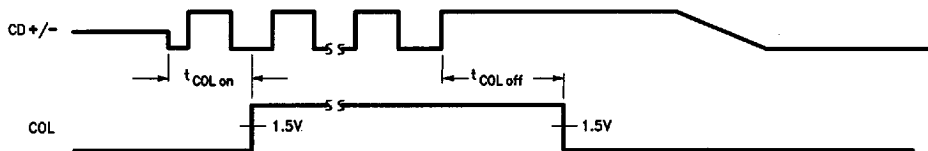
FIGURE 10. Collision Timing
