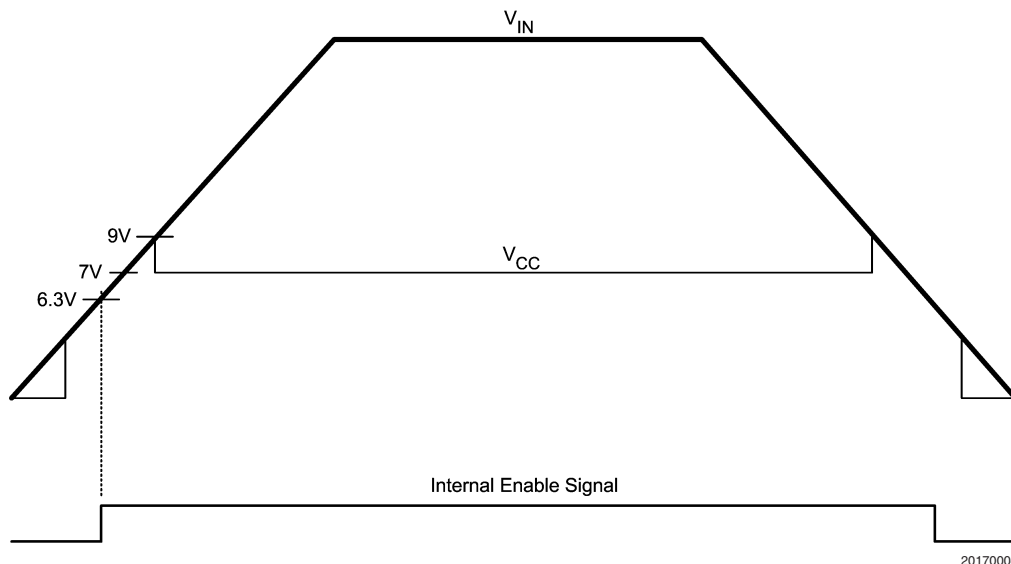
FIGURE 2. Vin and Vcc Sequencing
