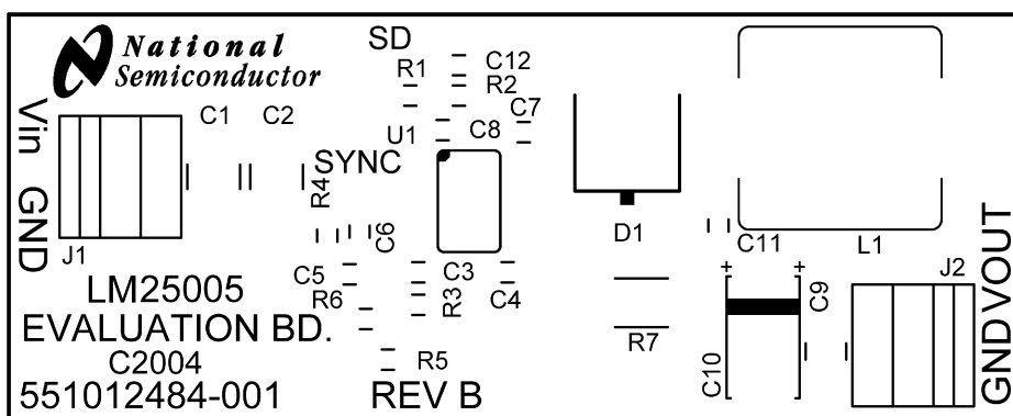
Silkscreen
