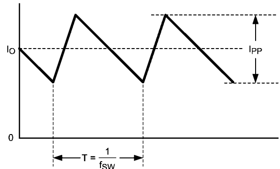
FIGURE 9. Inductor Current
