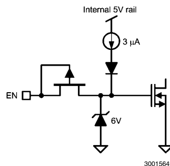
FIGURE 3. Enable Circuit
