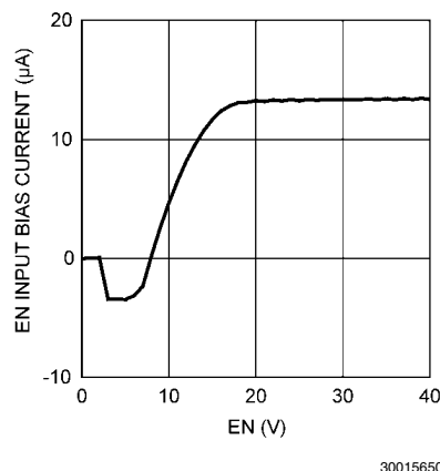
FIGURE 4. EN Bias Current vs Voltage
