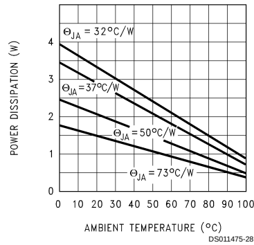
Maximum Power Dissipation (TO-263) (See (Note 12))
