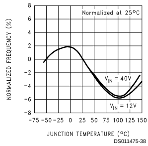
Oscillator Frequency
