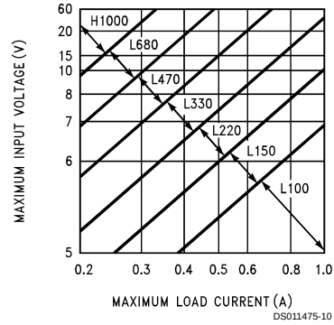
FIGURE 3. LM2575(HV)-3.3
