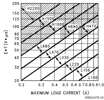
FIGURE 7. LM2575(HV)-ADJ
