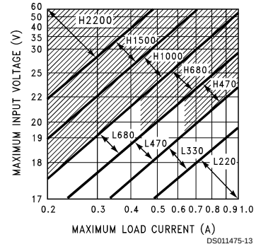
FIGURE 6. LM2575(HV)-15
