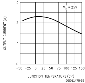
Current Limit
