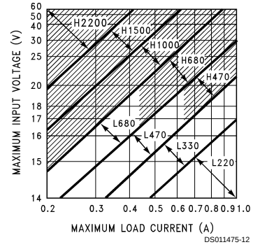
FIGURE 5. LM2575(HV)-12
