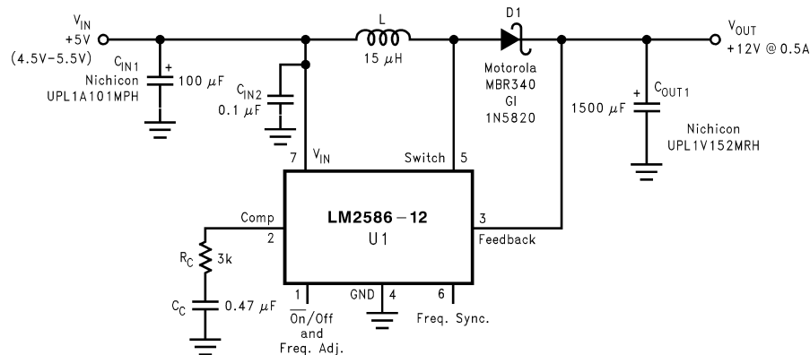
FIGURE 33. +5V to +12V Boost Regulator
