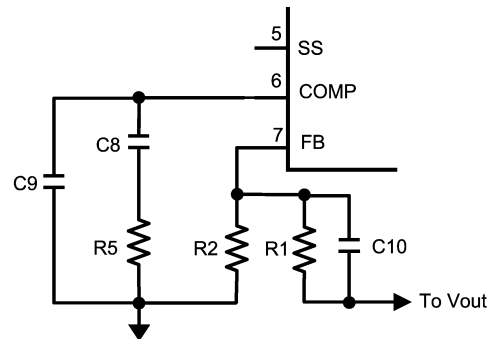
FIGURE 10. Compensation Network
