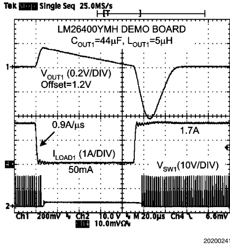
FIGURE 4. Extreme Load Step
