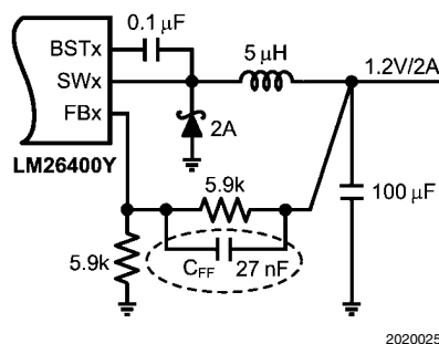
FIGURE 2. Adding a C_{FF} Capacitor
