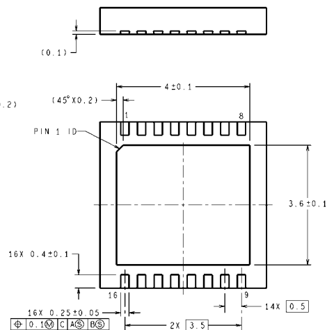
16-Lead LLP Package NS Package Number SDA16A
