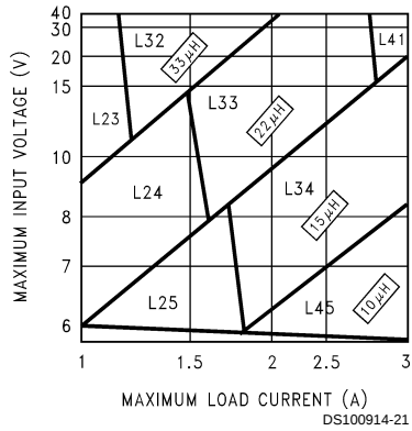
FIGURE 3. LM2676-3.3
