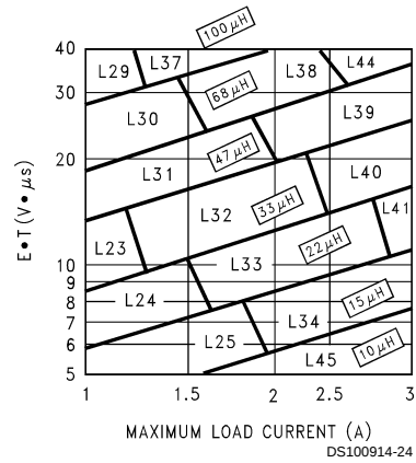
FIGURE 6. LM2676-ADJ
