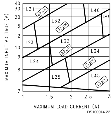
FIGURE 4. LM2676-5.0
