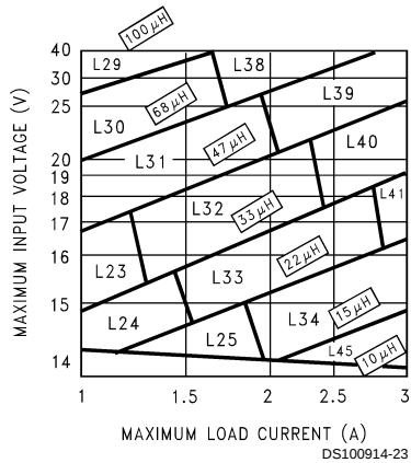
FIGURE 5. LM2676-12
